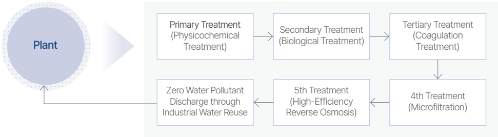
Jigok Plant Wastewater Treatment Flowchart
