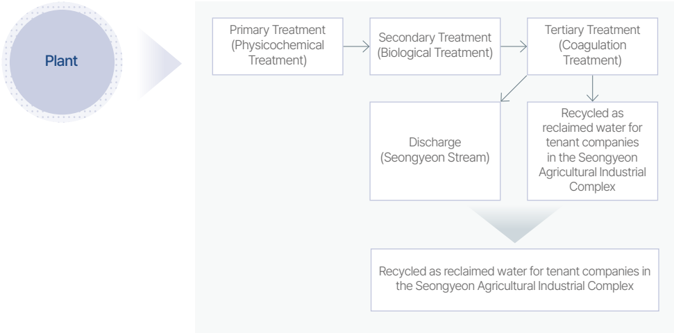
Seongyeon Plant Wastewater Treatment Flowchart
